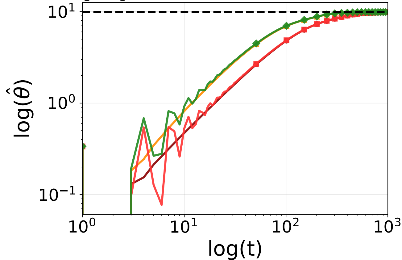
Log-Log Plot - D = 50, N = 20, X_0 \sim \mathcal{N}(0, 1)
